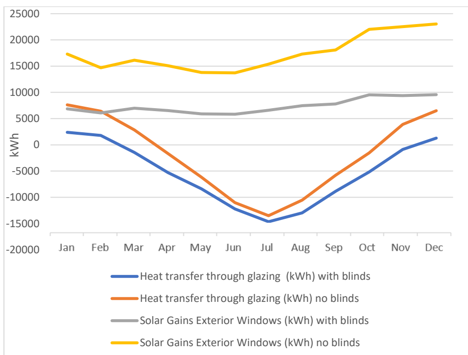
Figure 17: Heat transfer and solar gains with and without blinds
